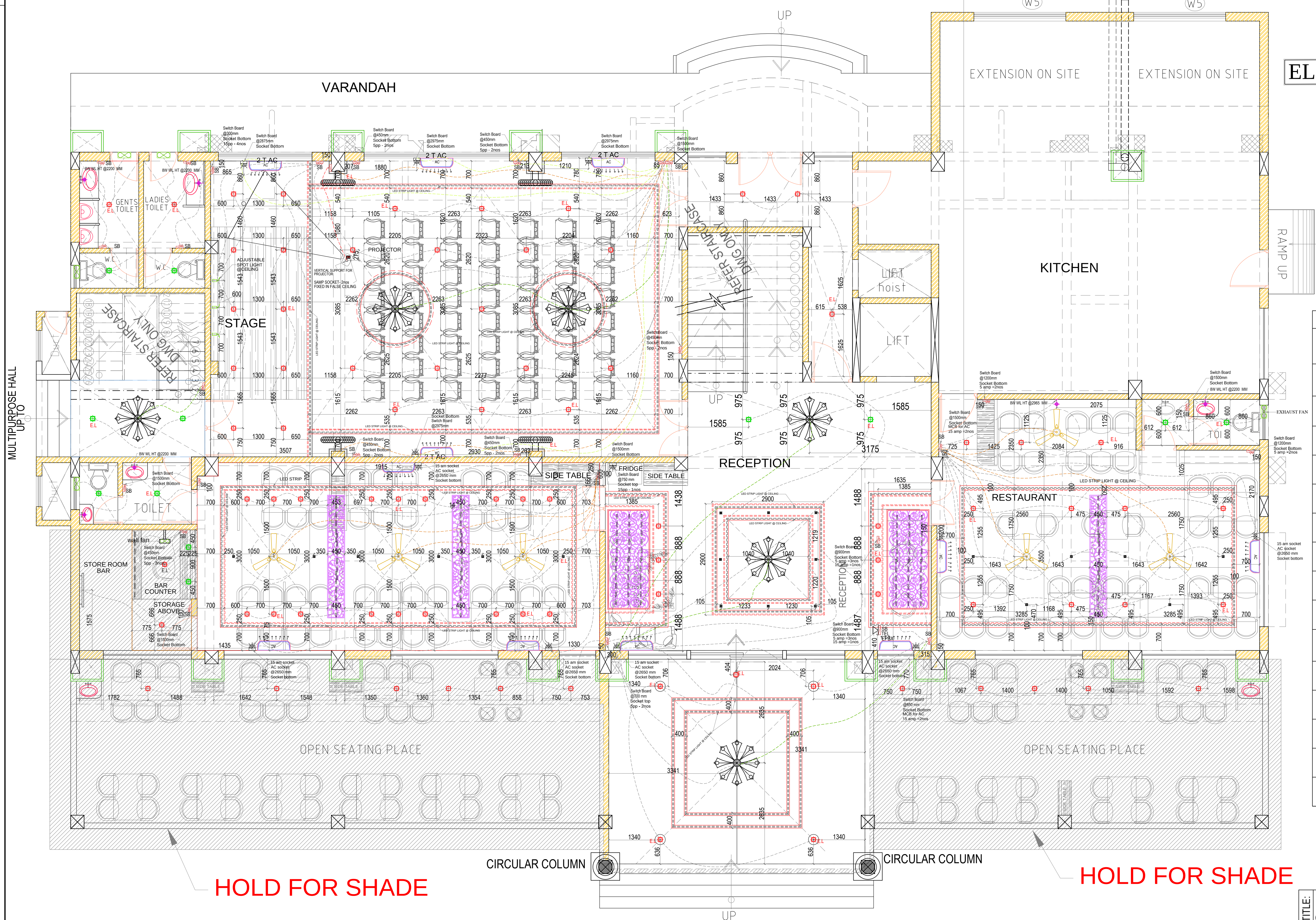
ELECTRICAL LAYOUT GROUND FLOOR
