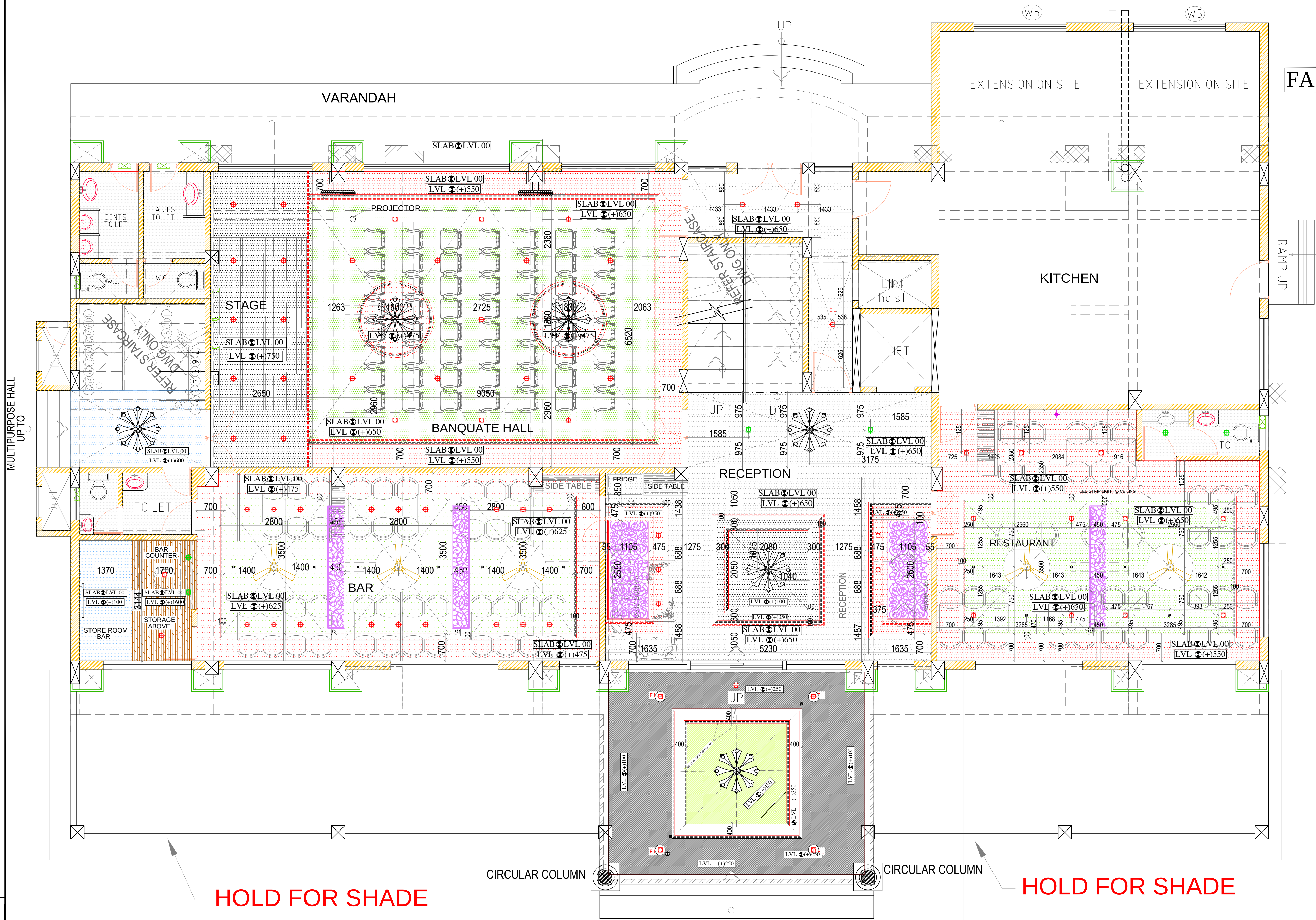
FASE CEILINGLAYOUT GROUND FLOOR
